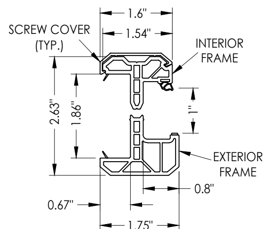
5A ODL KEYSTONE PVC LITE FRAME 1" GLAZING
