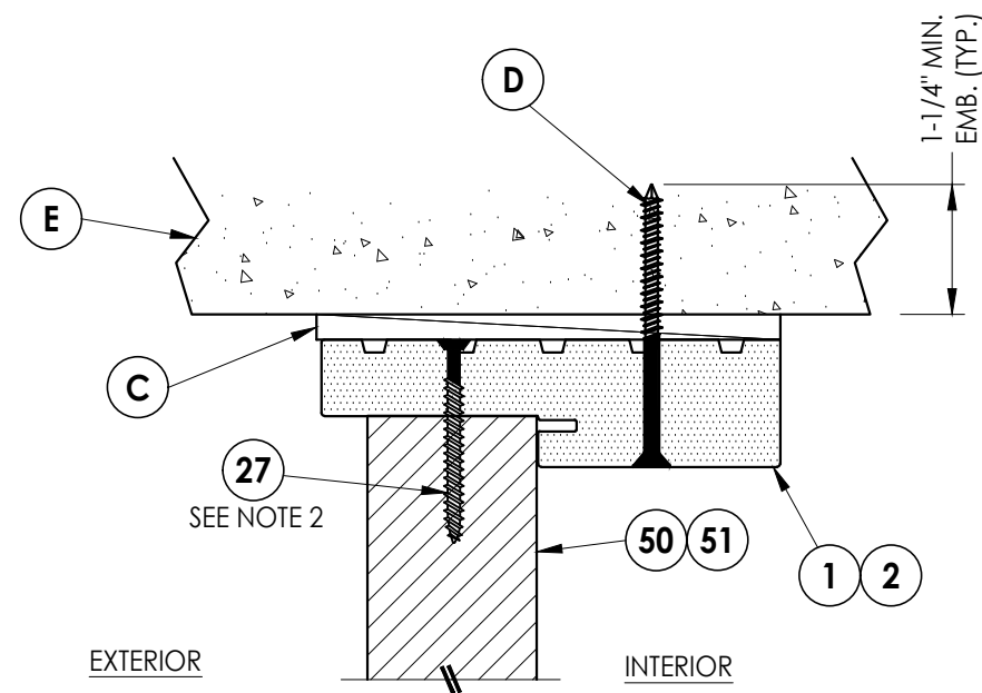
3 VERTICAL CROSS SECTION 10 Outswing Shown (Inswing Similar) Shown Direct to Masonry
