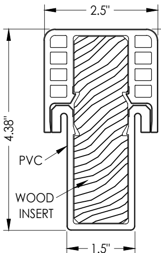
3 COMPOSITE MULLION ENDURA FUSION w/ PVC Boot
