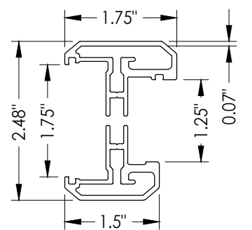
4B ODL FLAT ALUMINUM LITE FRAME 1-1/4" GLAZING
