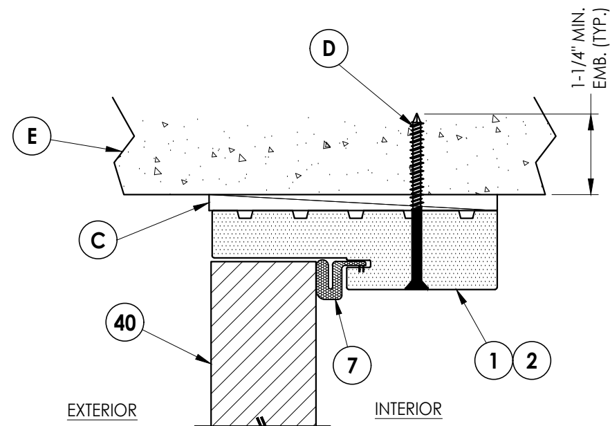
2 VERTICAL CROSS SECTION 10 Outswing Shown (Inswing Similar) Shown Direct to Masonry
