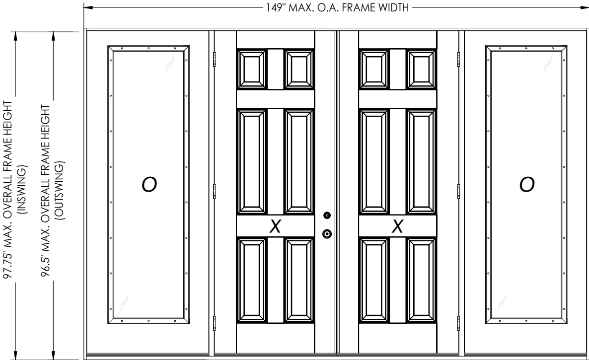
OXXO CONTINUOUS HEAD & SILL
